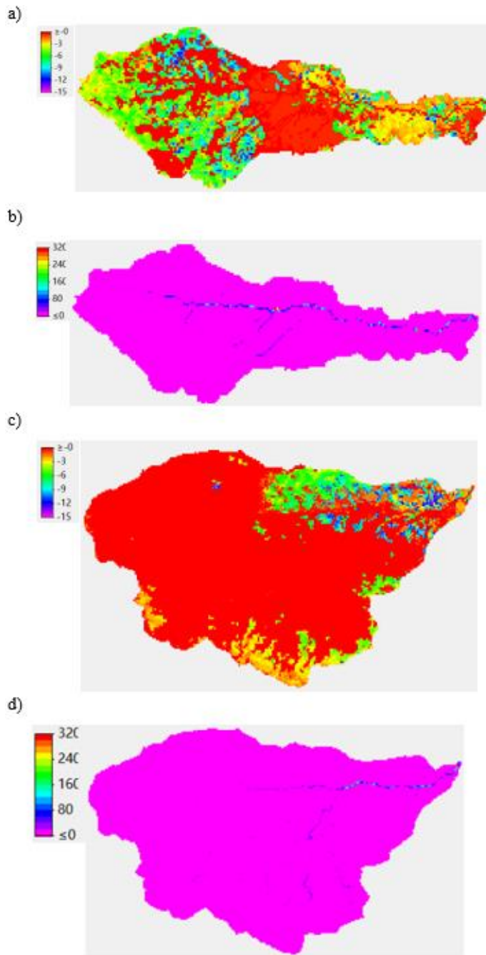
Figure 5.4 Spatial explicit of annual soil loss and deposition of two watersheds in 2014: a) referring to soil loss in S1 watershed; b) referring to deposition in S1 watershed; c) referring to soil loss in S2 watershed; d) referring to deposition in S2 watershed
