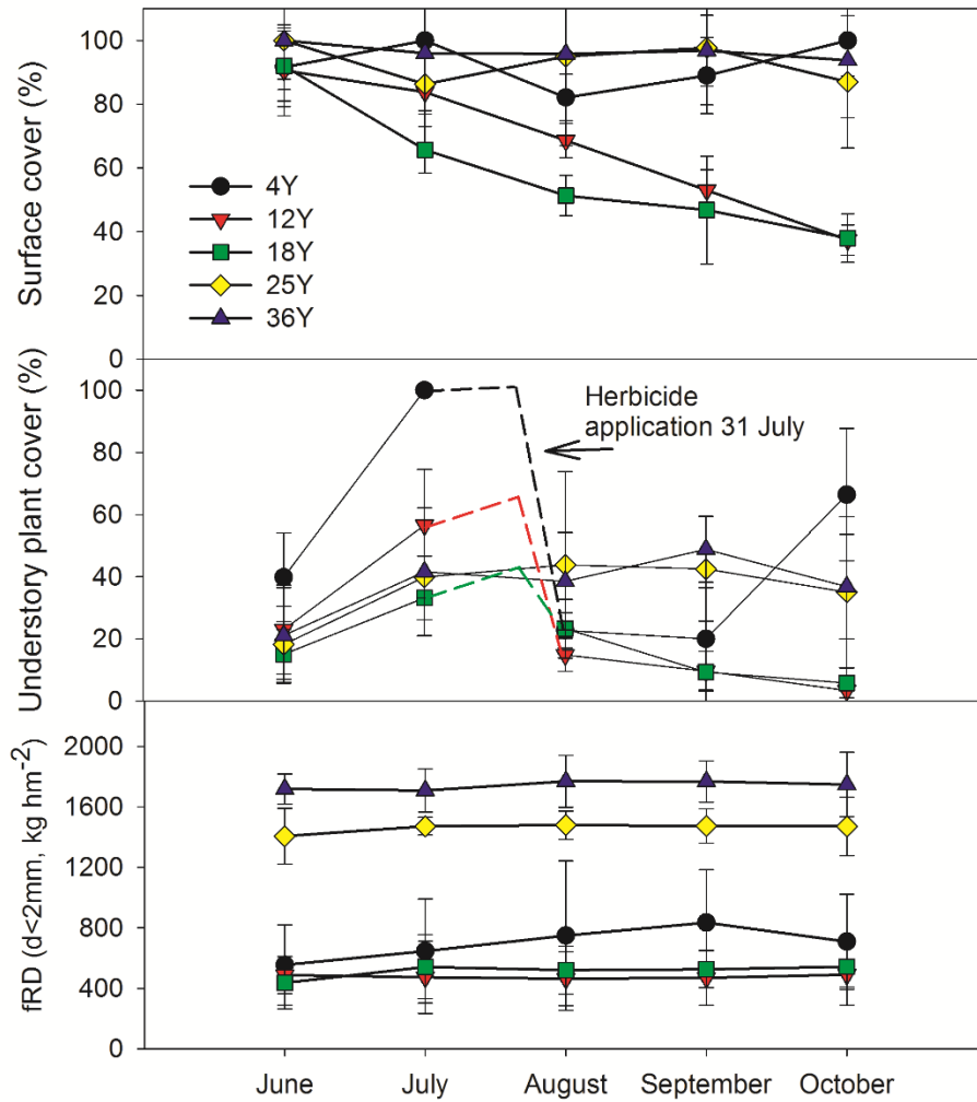
Figure 2.5 Temporal dynamics of (a) surface cover (understory plant and litter cover), (b) understory plant cover, (c) fine roots content ( d < 2 mm) under different rubber ages from June to October in 2014.
